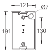
Mounting detail
